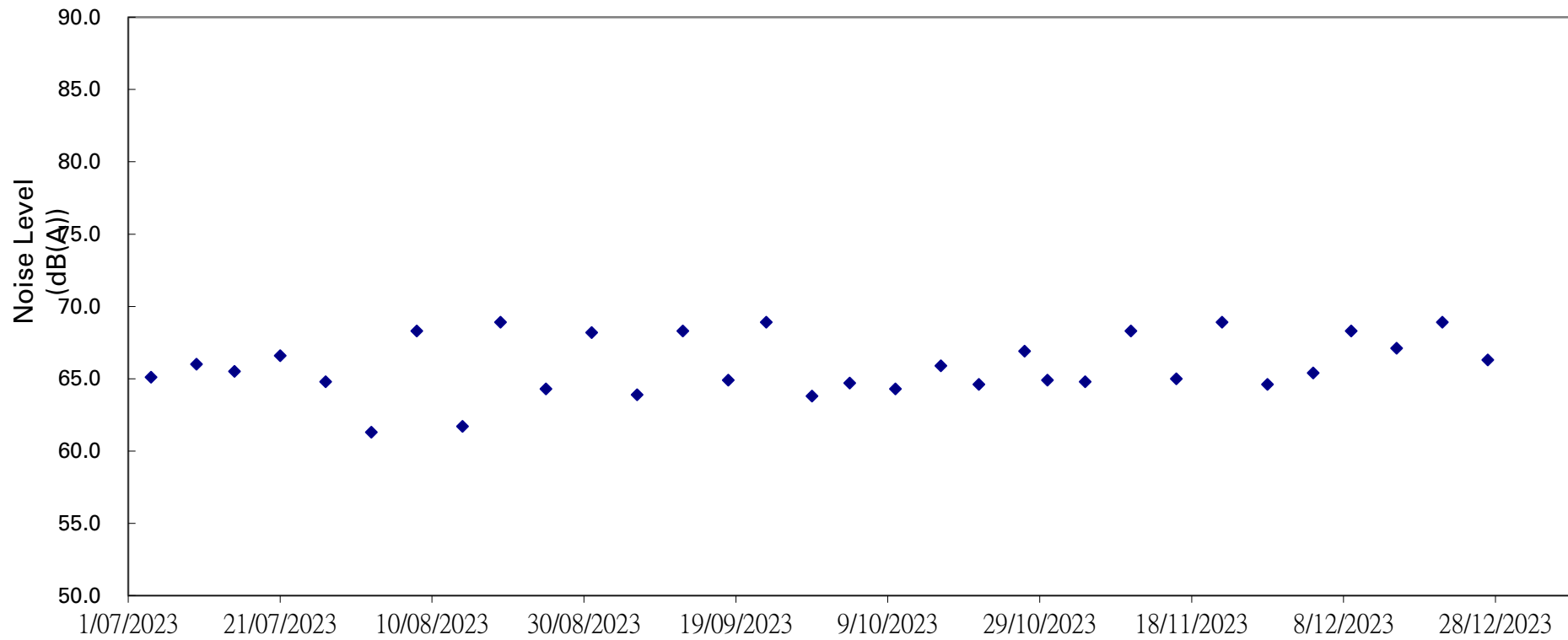
Noise Level (Leq 30 mins) dB(A) Vs Date for Location W-P11
